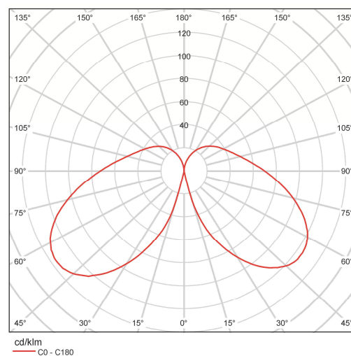
Courbe de distribution KARIN 1200 LED
